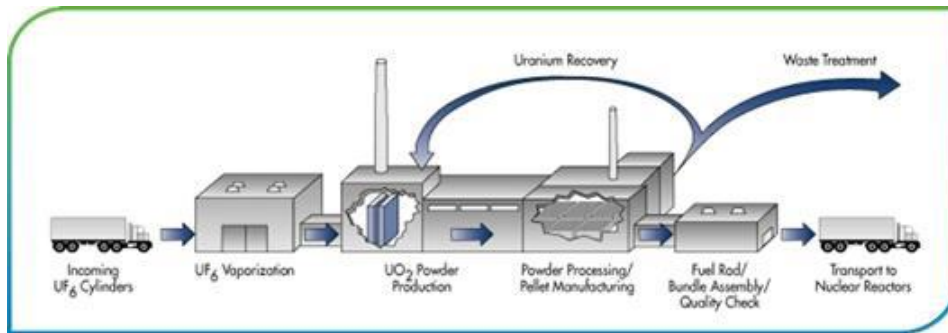
Proposed HALEU Fuel Processing Facility
